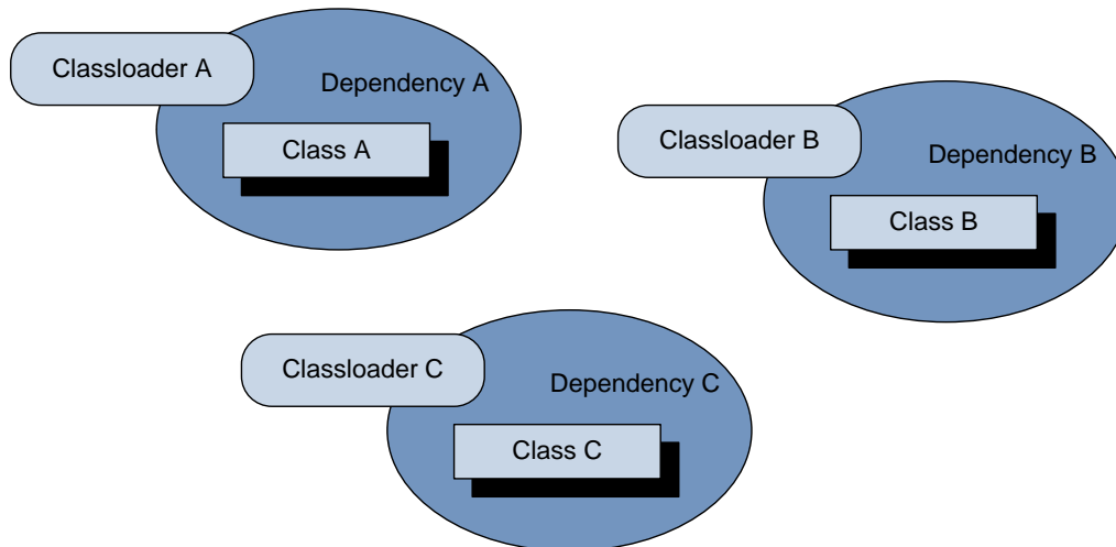
Figure 8: Dependency classloaders
